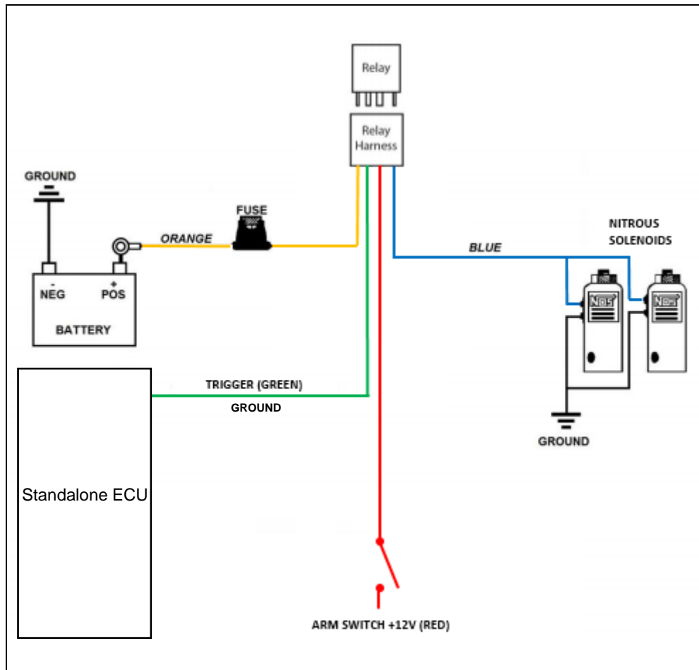
Figure 14 – Relay Wiring
