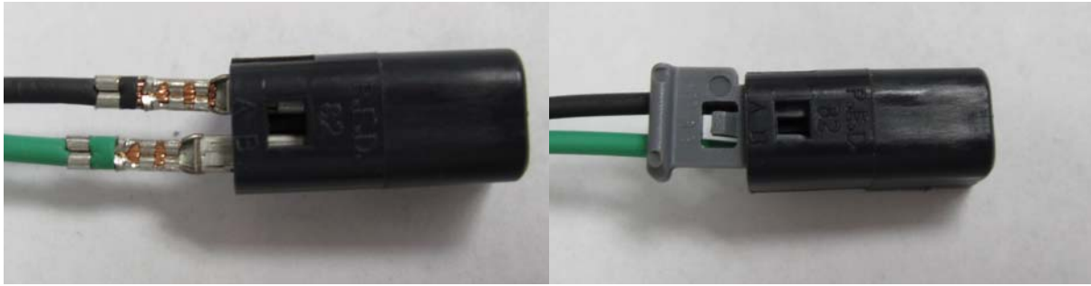
Figure 1. Insert Terminals and Lock
