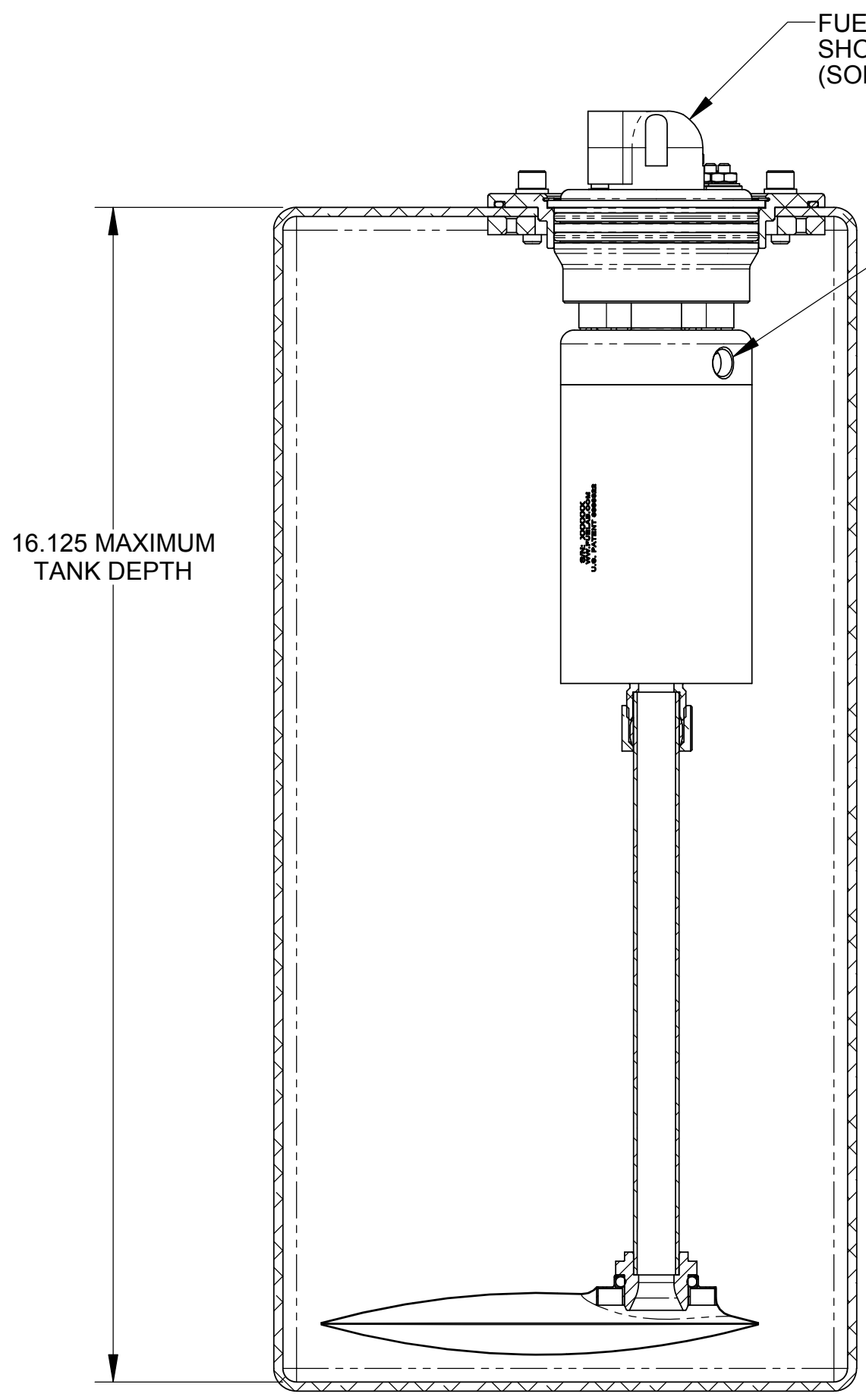
MAXIMUM INSTALLATION HEIGHT SHOWN ABOVE SCALE: 1/2
