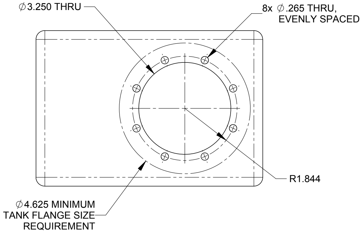
TANK FABRICATION REQUIREMENT SHOWN ABOVE SCALE: 1/2
