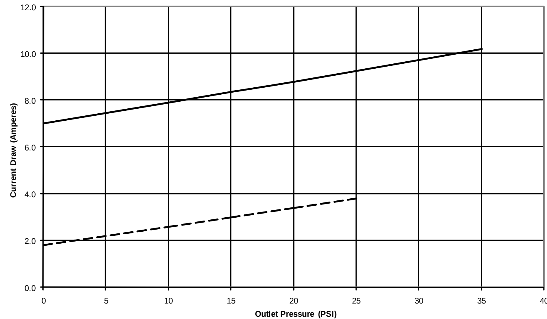
Current Draw Performance - Model 90902, at 13.5 Volts
