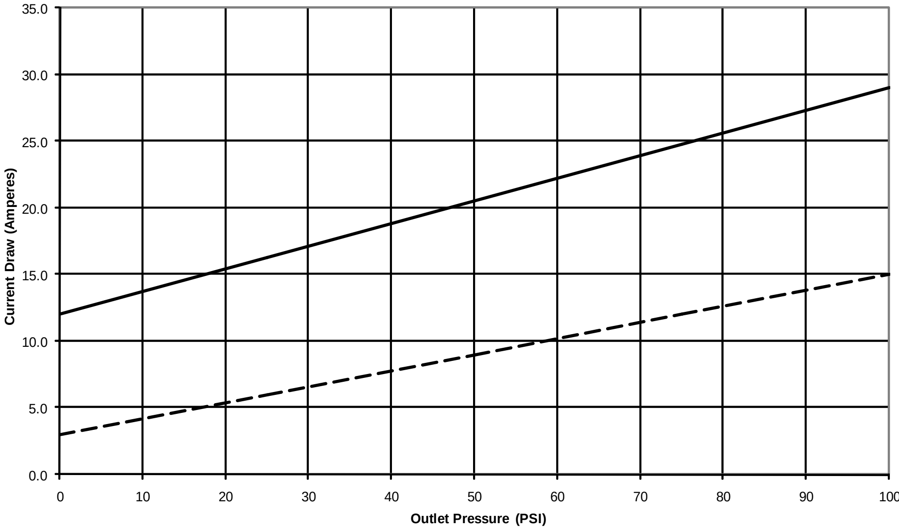
Current Draw Performance - Model 92902, at 13.5 Volts
