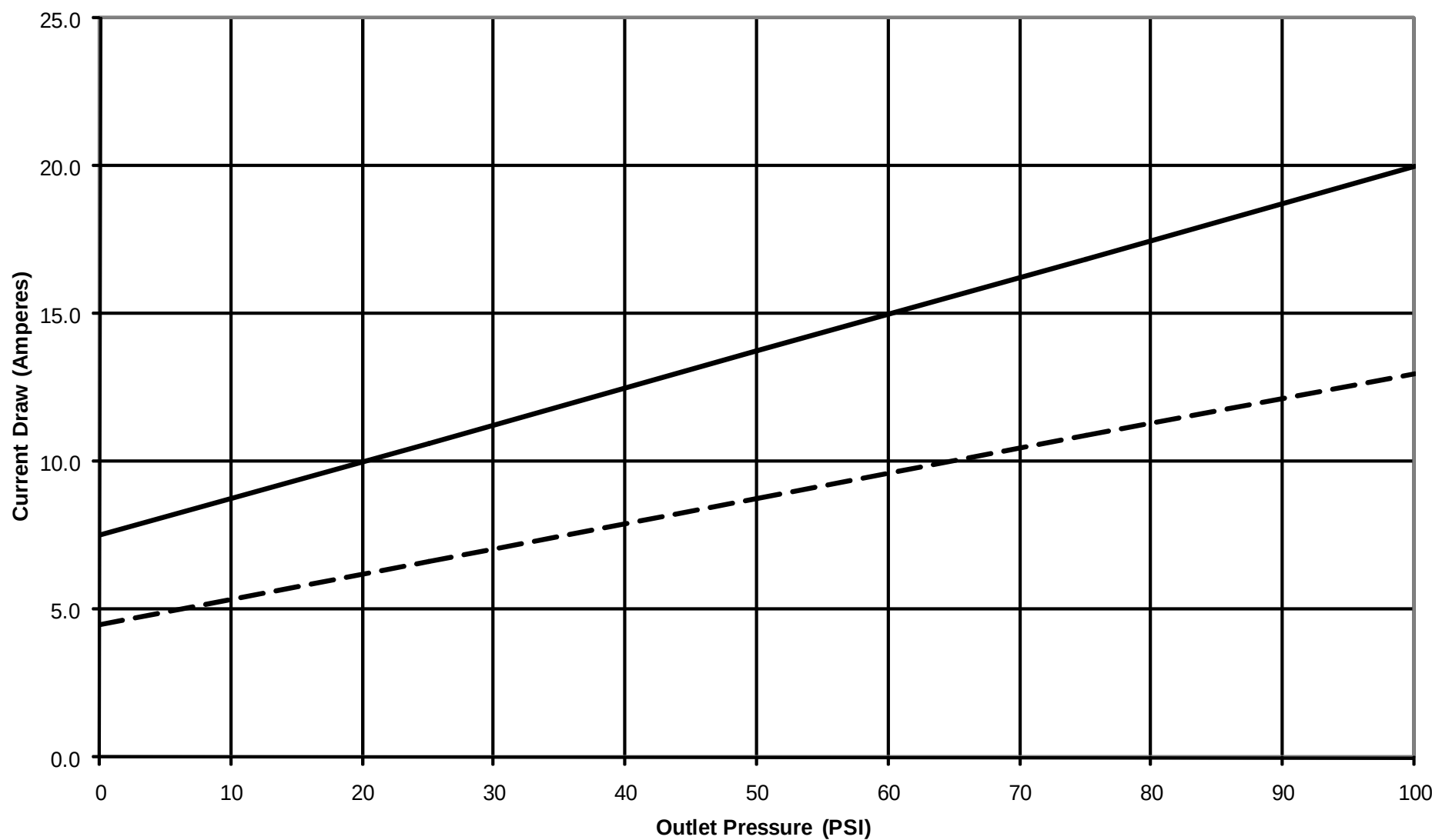
Current Draw Performance - Model 91901, at 13.5 Volts
