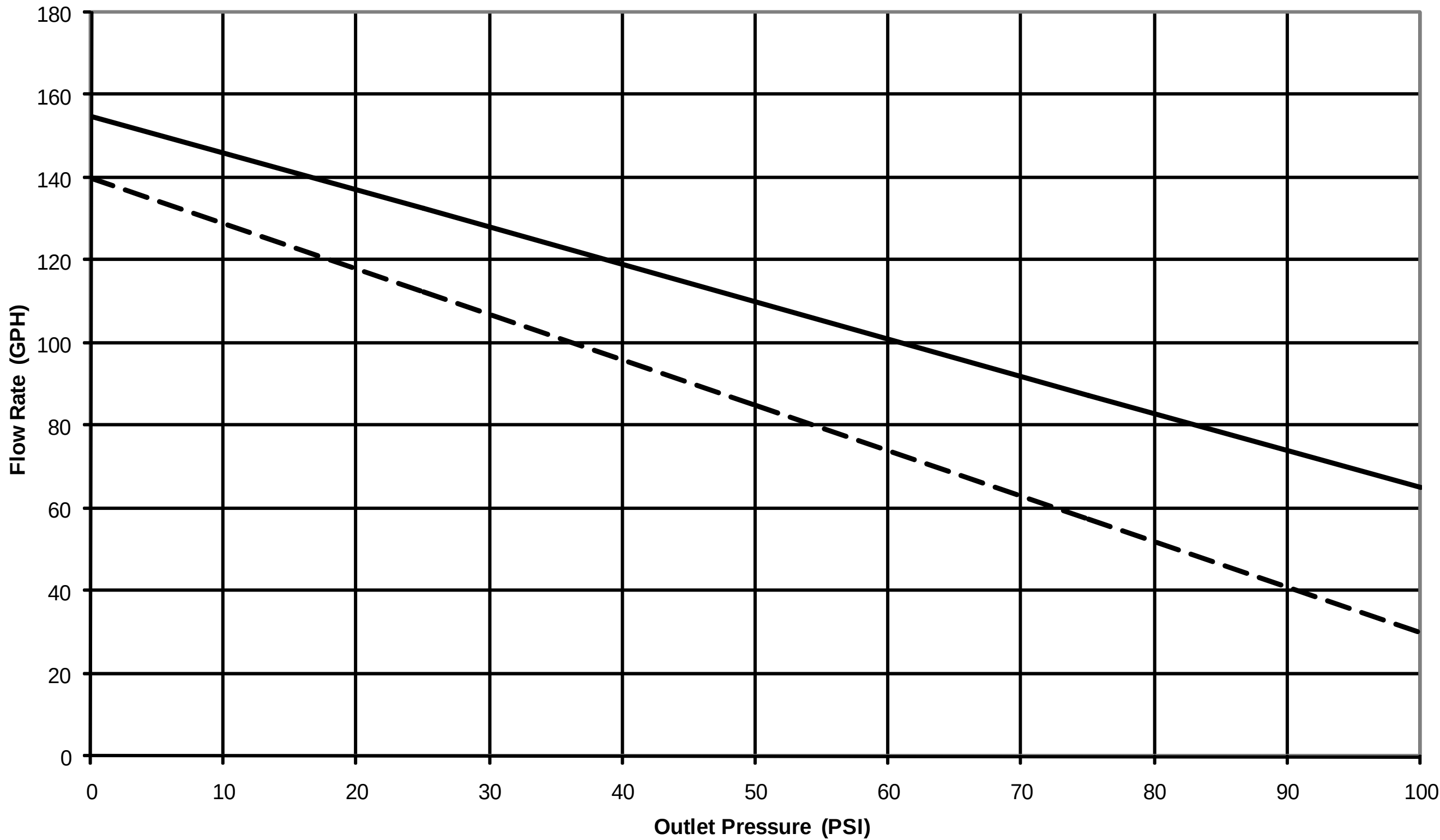
Flow Performance - Model 91901, at 13.5 Volts
