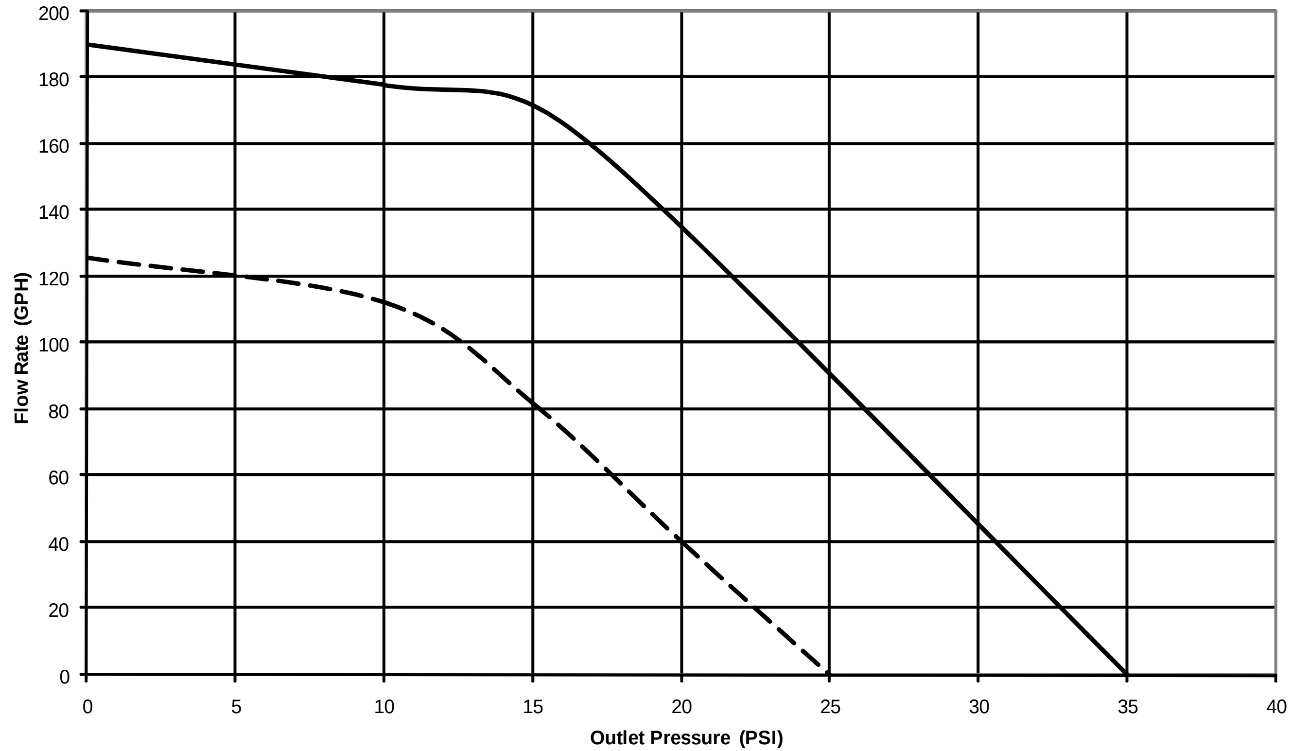
Flow Performance - Model 90902, at 13.5 Volts
